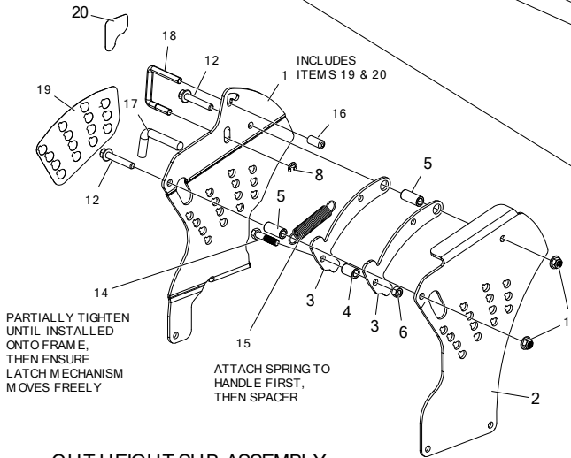
CUT HEIGHT SUB-ASSEMBLY
