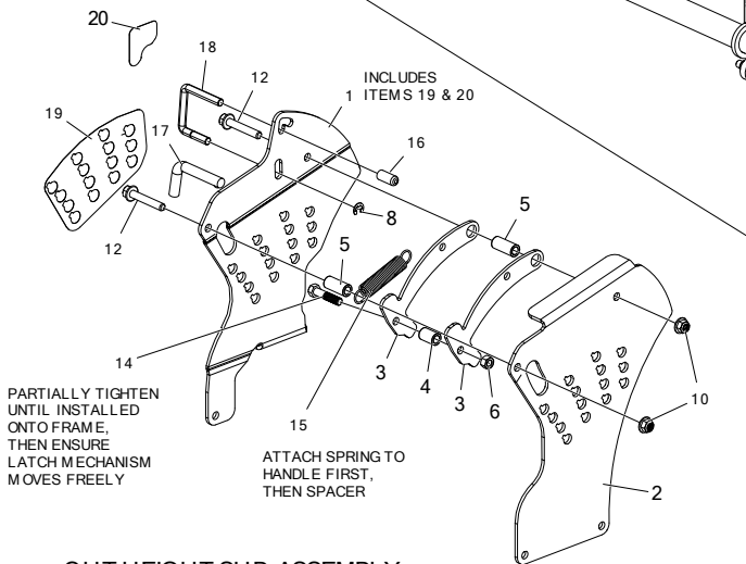
CUT HEIGHT SUB-ASSEMBLY
