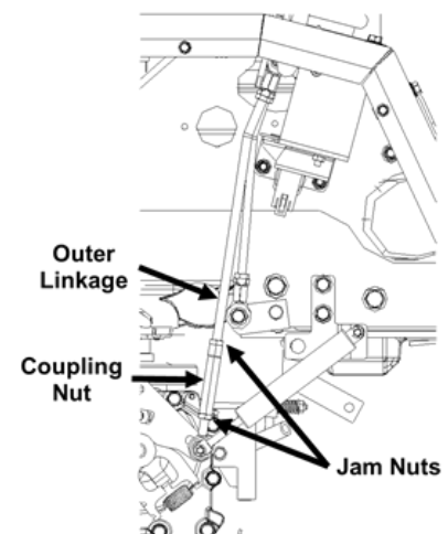
Right Side Transmission
