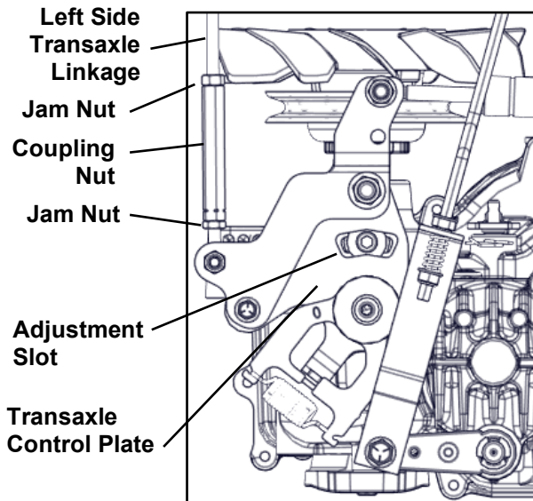
Left Side Transaxle
