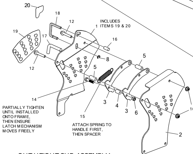
CUT HEIGHT SUB-ASSEMBLY
