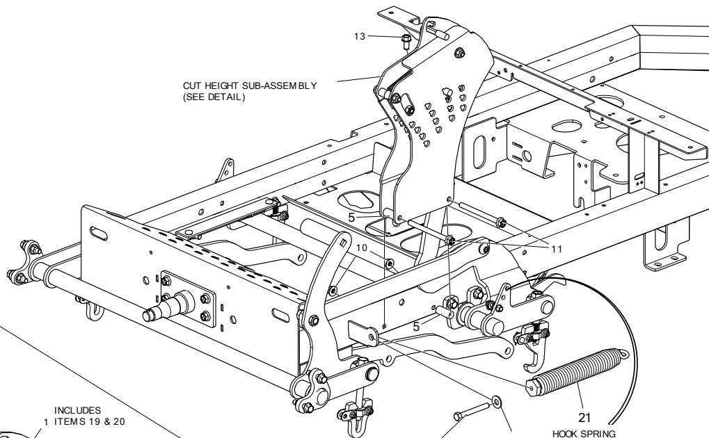
HOCK SPRING (WITH HOOK ON TOP) IN TOP HOLE - 52" & 60" DECK BOTTOM HOLE - 48" DECK
