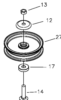
FRONT STATIONARY IDLER ASSEMBLY
