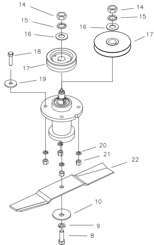
609F-019A USED ON 42" TRI-PORT DECK ASSEMBLY (686A-002A)
