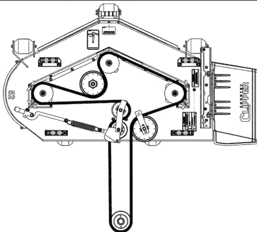
Charger 52" Deck Belt Routing
