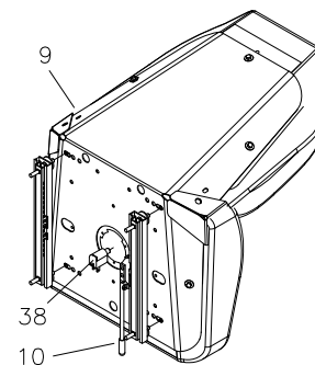
SEAT ASS'Y
