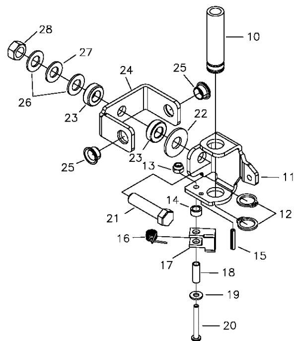
YOKE, SWIVEL ASSEMBLY {625-129A}
