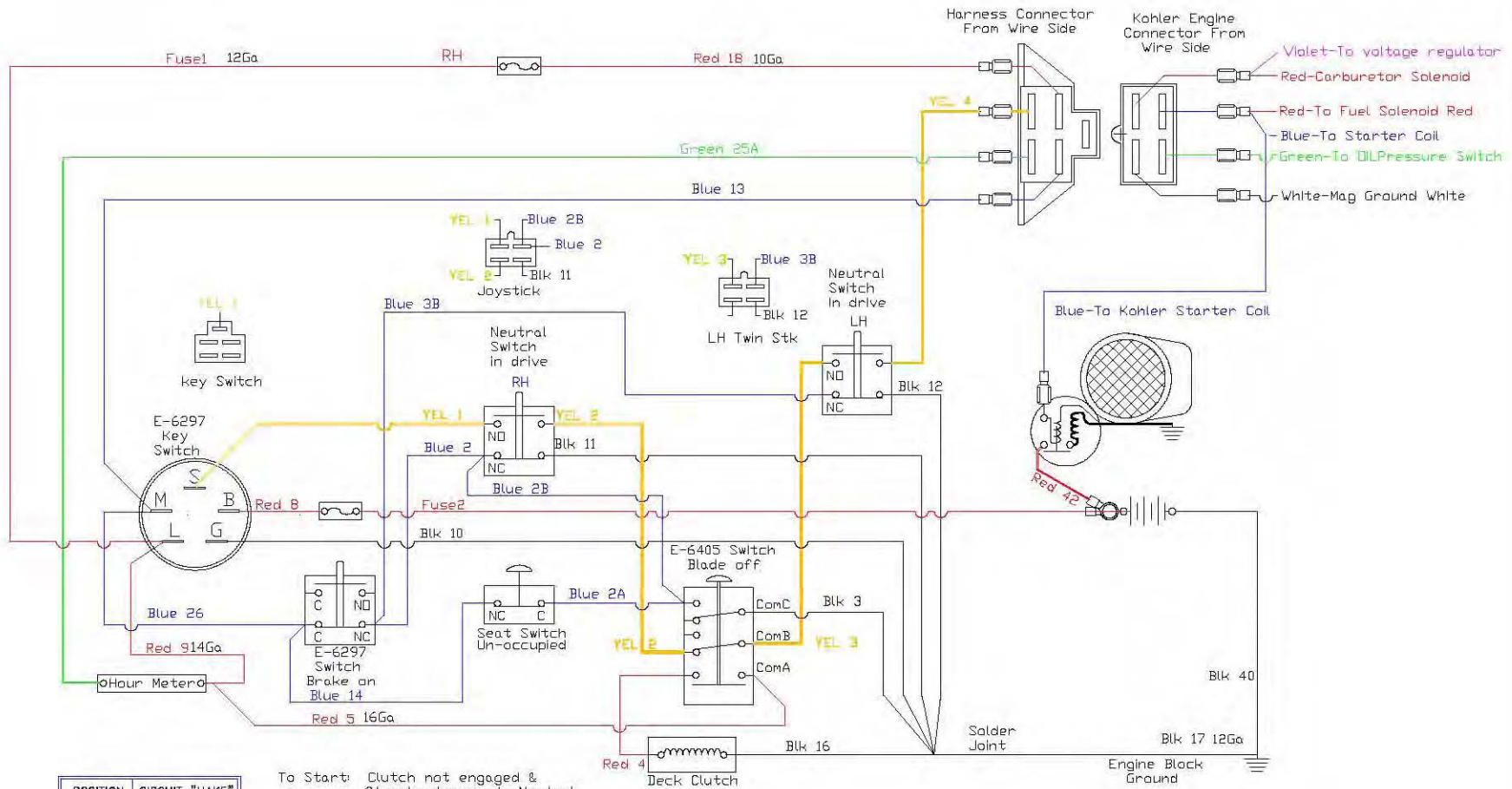
WIRING SCHEMATIC FOR KOHLER TWINSTICK (E-6416)
