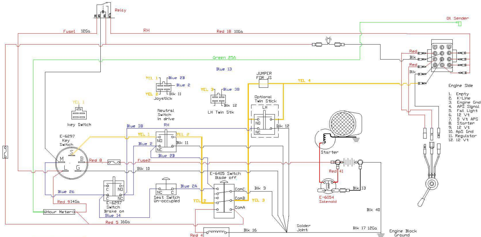
E-6472-Boss Kawasaki DFI Harness 7-30-10 PWR
