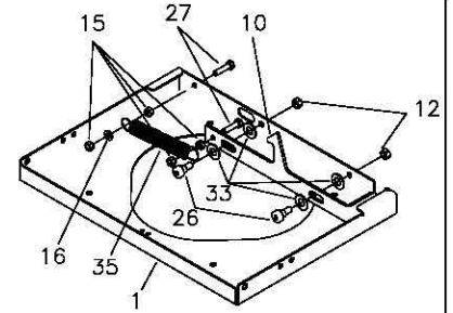
UNDERSIDE OF SEAT MOUNTING BASE "#1" - LATCH PARTS
