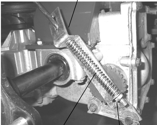
Brake Adjustment Spring
